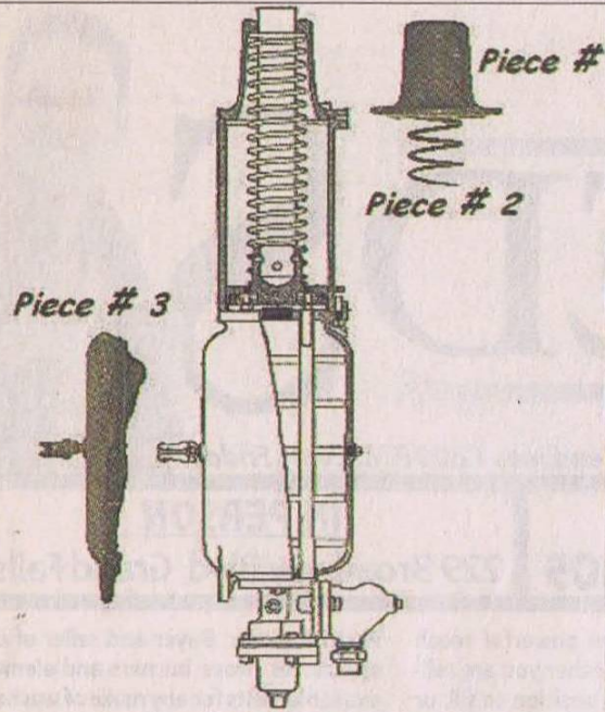
LOCOMOTIVE ENGINEERING FIGURE 238.—TRIPLE VALVE, AUXILIARY RESERVOIR AND BRAKE CYLINDER COMBINED
